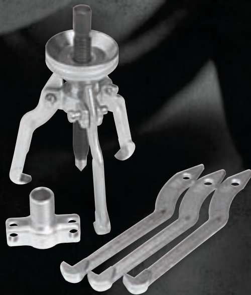
6 TON PROTO-EASE™ 2-WAY/3-WAY CONE PULLER SET
